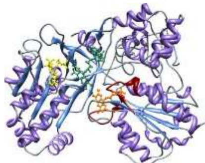
Cytochrome P450
